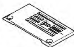
14-744 3/16" 14-754 7/32" 14-764 1/4" Needle plate
