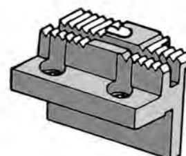
240093 Feed Dog 11 Teeth, 15 Teeth to 1"
