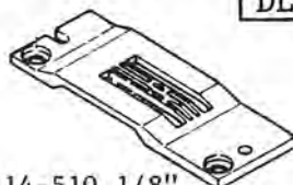
14-510 1/8" 14-511 3/16" 14-512 1/4" Needle plate
