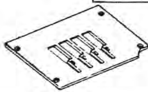
Needle plate 14-421 1" 14-422 1-1/8" 14-423 1-1/4" 14-424 1-1/2"
