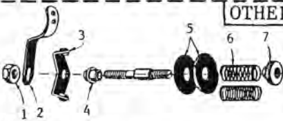
5127H (G52827-16) Presser foot
