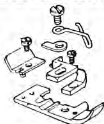
202173-3-10 presser foot
