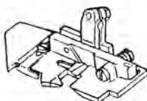
204706-3-12 (204706-3-11) Foot comp.
