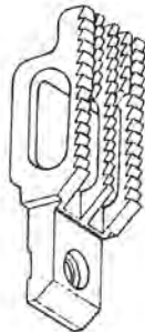
139382 1/4" Feed Dog 14 teeth 10 teeth to 1"
