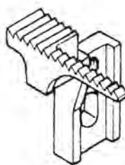
20461 Main Feed Dog
