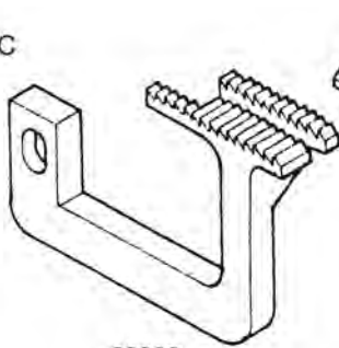
33828 Differential Feed Dog
