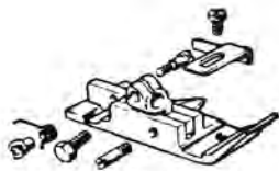
205034-3-12 (205034-3-11) Foot comp.
