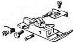
204875-3-12 (204875-3-11) Foot comp.
