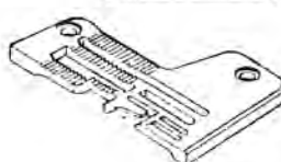
203035-0-11 Needle plate
