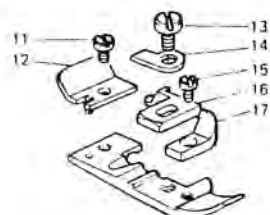
202171-3-10 presser foot
