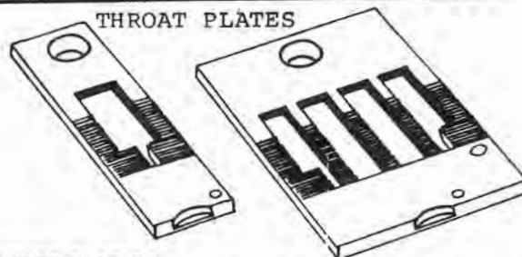
THROAT PLATES
